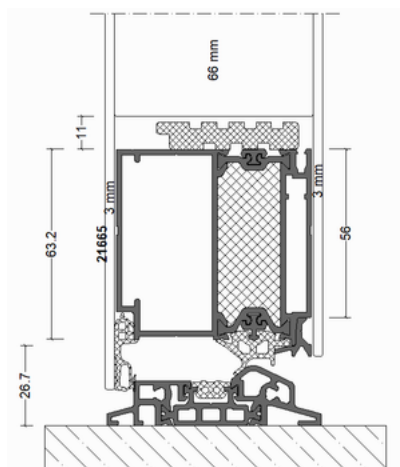
Low level threshold detail
