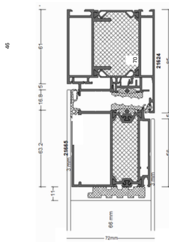
Frame/Sash section detail
