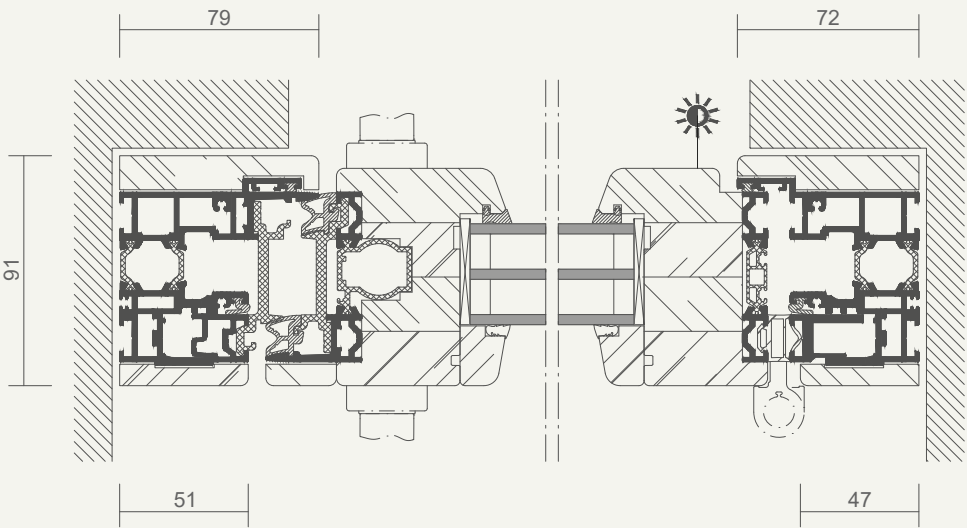
Horizontal section
