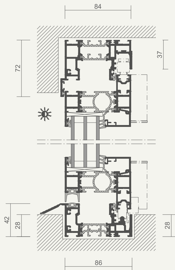
Vertical section
